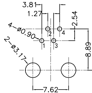
RECOMMENDED PCB LAYOUT VIEWED FROM COMPONENT SIDE
