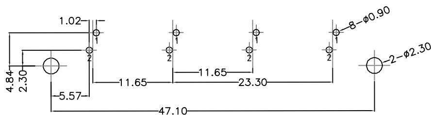
RECOMMENDED PCB LAYOUT VIEWED FROM COMPONENT SIDE
