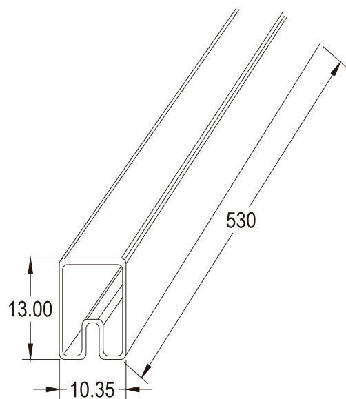
Tube: 530*13.0*10.35mm
