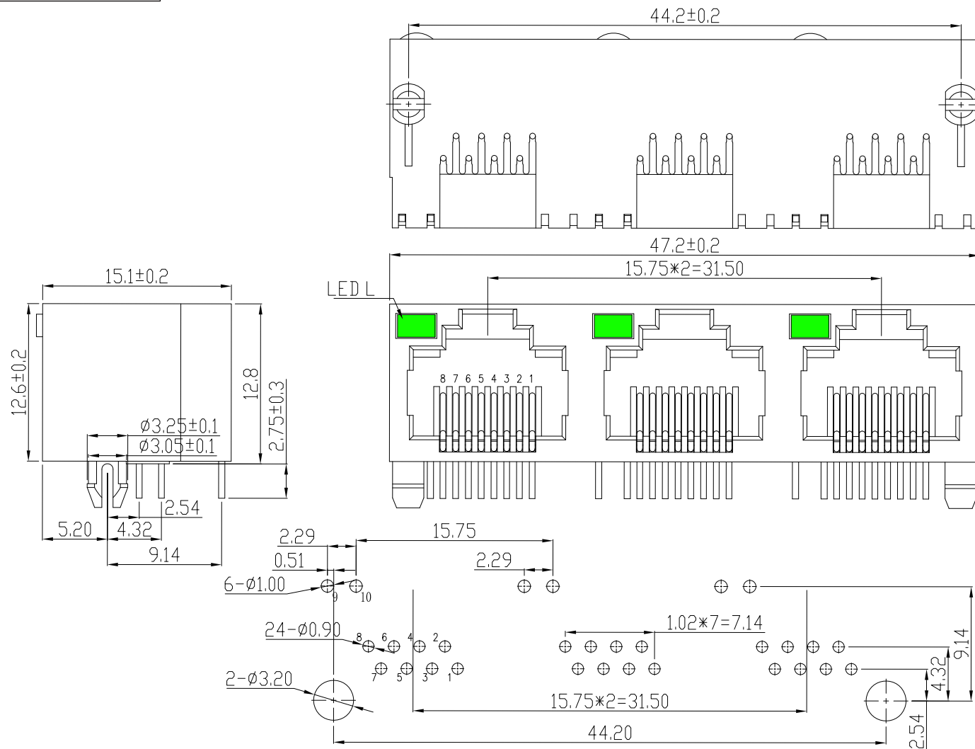
PC Board Layout
