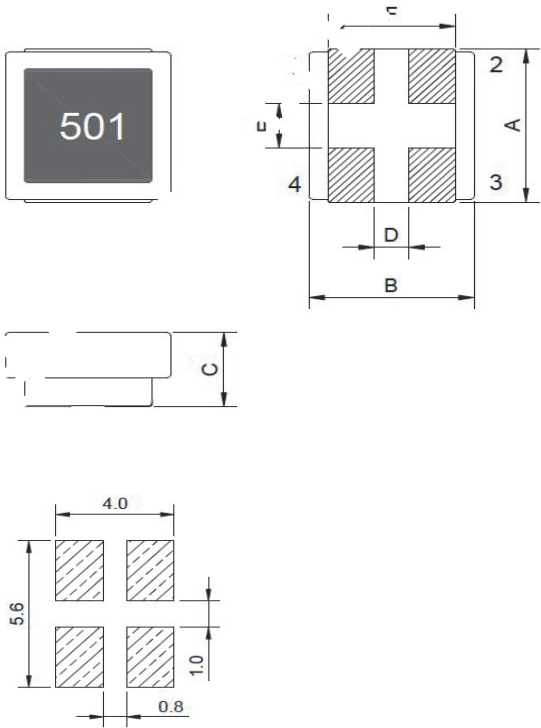
Reference land pattern (mm)
