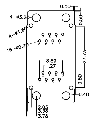
RECOMMENDED PCB LAYOUT VIEWED FROM COMPONENT SIDE
