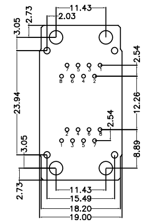
RECOMMENDED PCB LAYOUT VIEWED FROM COMPONENT SIDE
