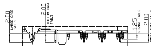
DETAIL A SCALE 2:1
