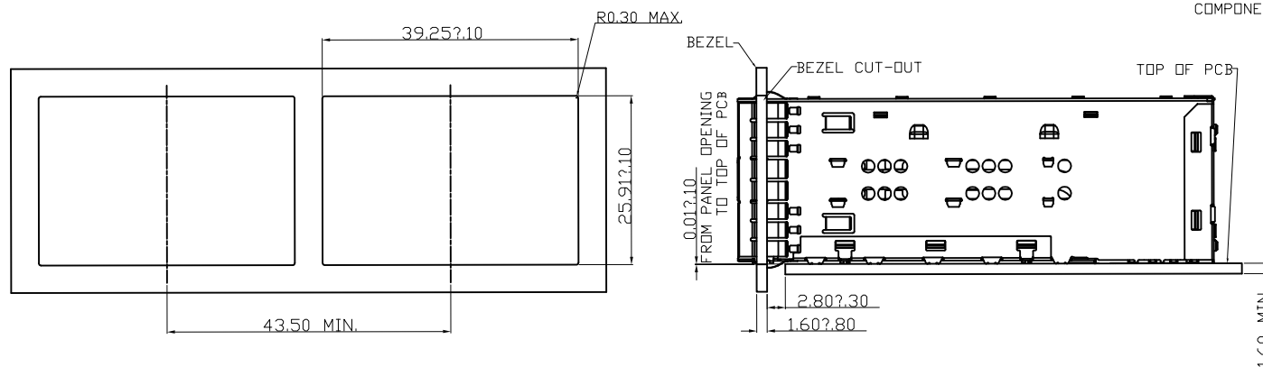
RECOMMENDED PANEL-CUT OUT
