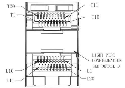
DETAIL A1 SCALE 4:1
