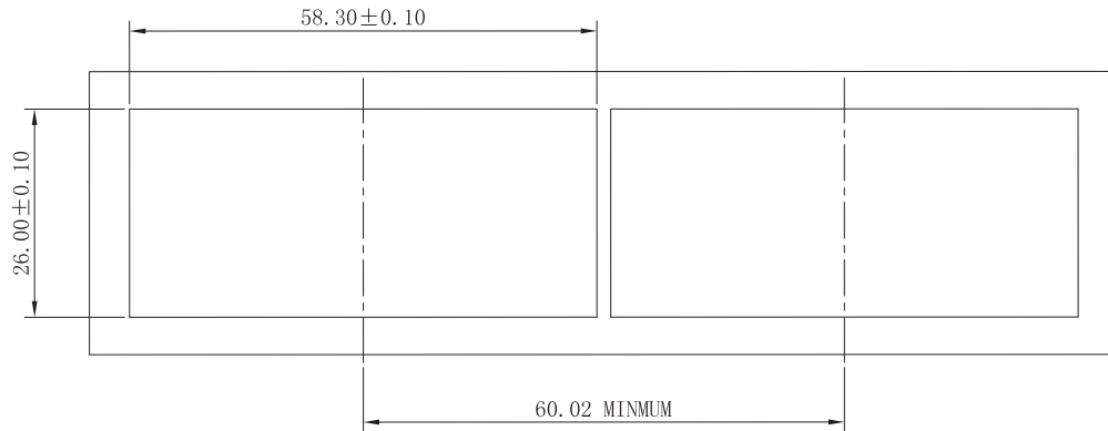
BEZEL CUT-OUT CENTER SPACING DETAIL BEZEL THICKNESS:0.8-2.6
