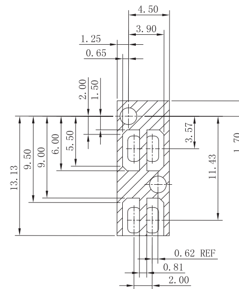
KEEPOUT ZONE DETAIL SCALE 5:1
