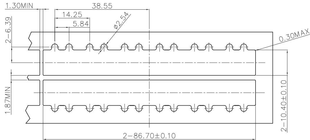
BEZEL RECOMMENDED PANEL CUTOUT AND PC BOARD PANEL POSITION AND THICKNESS 0.8–2.6
