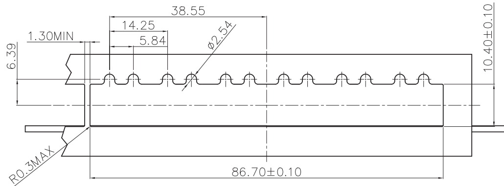
BEZEL RECOMMENDED PANEL CUTOUT AND PC BOARD PANEL POSITION AND THICKNESS 0.8–2.6
