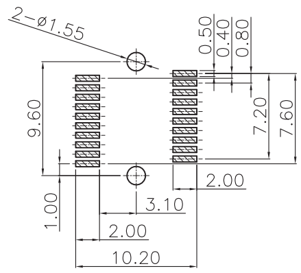
DETAIL A(SCALE 2:1)
