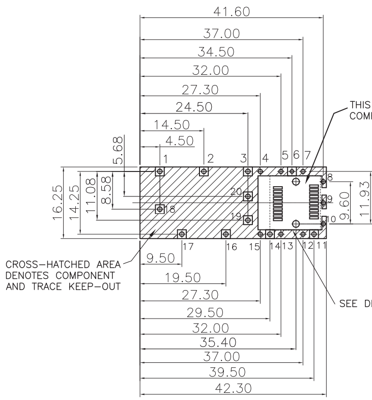
RECOMMENDED PCB LAYOUT (TOP VIEW) (ALL TOLERANCES ARE ±0.05)
