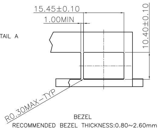
DETAIL A(SCALE 2:1)
