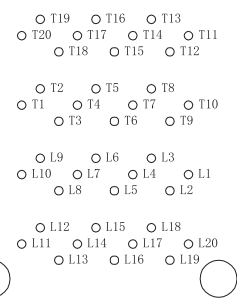
DETAIL D SCALE 2:1
