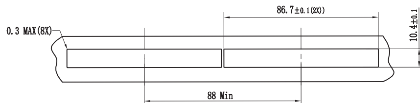
RECOMMENDED BEZEL CUT-OUT SINGLE SIDED APPLICATIONS SCALE 5:3
