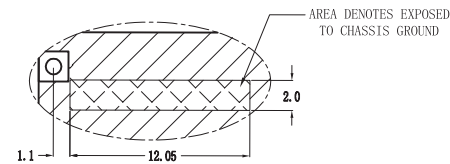
DETAIL D SCALE 3:1
