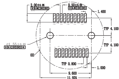
DETAIL C SCALE 3:1
