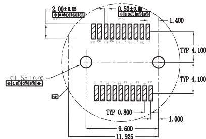
DETAIL E SCALE 3:1
