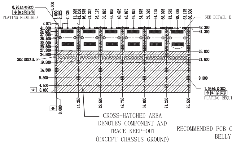
RECOMMENDED PCB CONFIGURATION WITH KEEP-OUT AREAS SINGLE SIDED APPLICATONS
