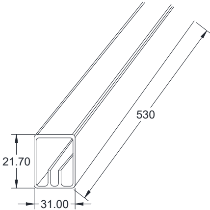
Tube: 530*31.00*21.70mm
