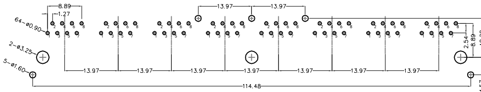
RECOMMENDED PCB LAYOUT VIEWED FROM COMPONENT SIDE
