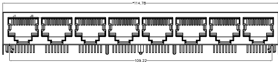
FRONT VIEW
