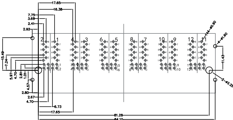
RECOMMENDED PCB LAYOUT VIEWED FROM COMPONENT SIDE
