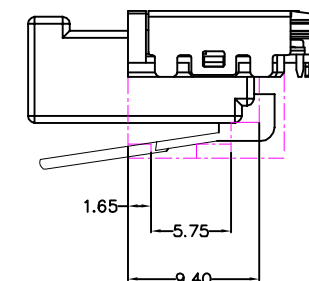
CONN.W/OPENING BASE W/PLUG DRAWING
