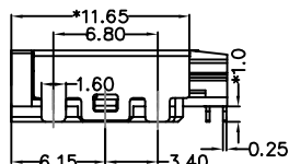
RIGHT SIDE VIEW
