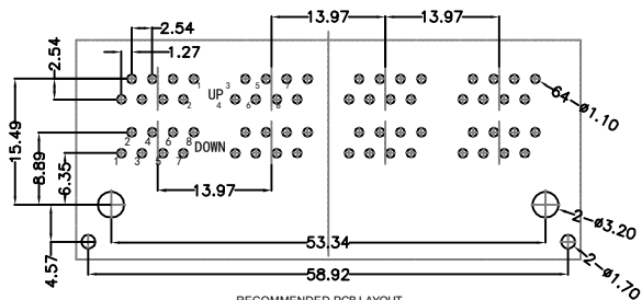
RECOMMENDED PCB LAYOUT VIEWED FROM COMPONENT SIDE
