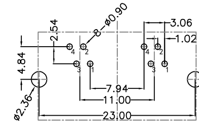
RECOMMENDED PCB LAYOUT VIEWED FROM COMPONENT SIDE
