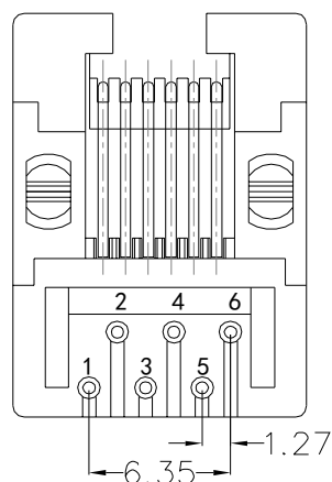
BOTTOM VIEW
