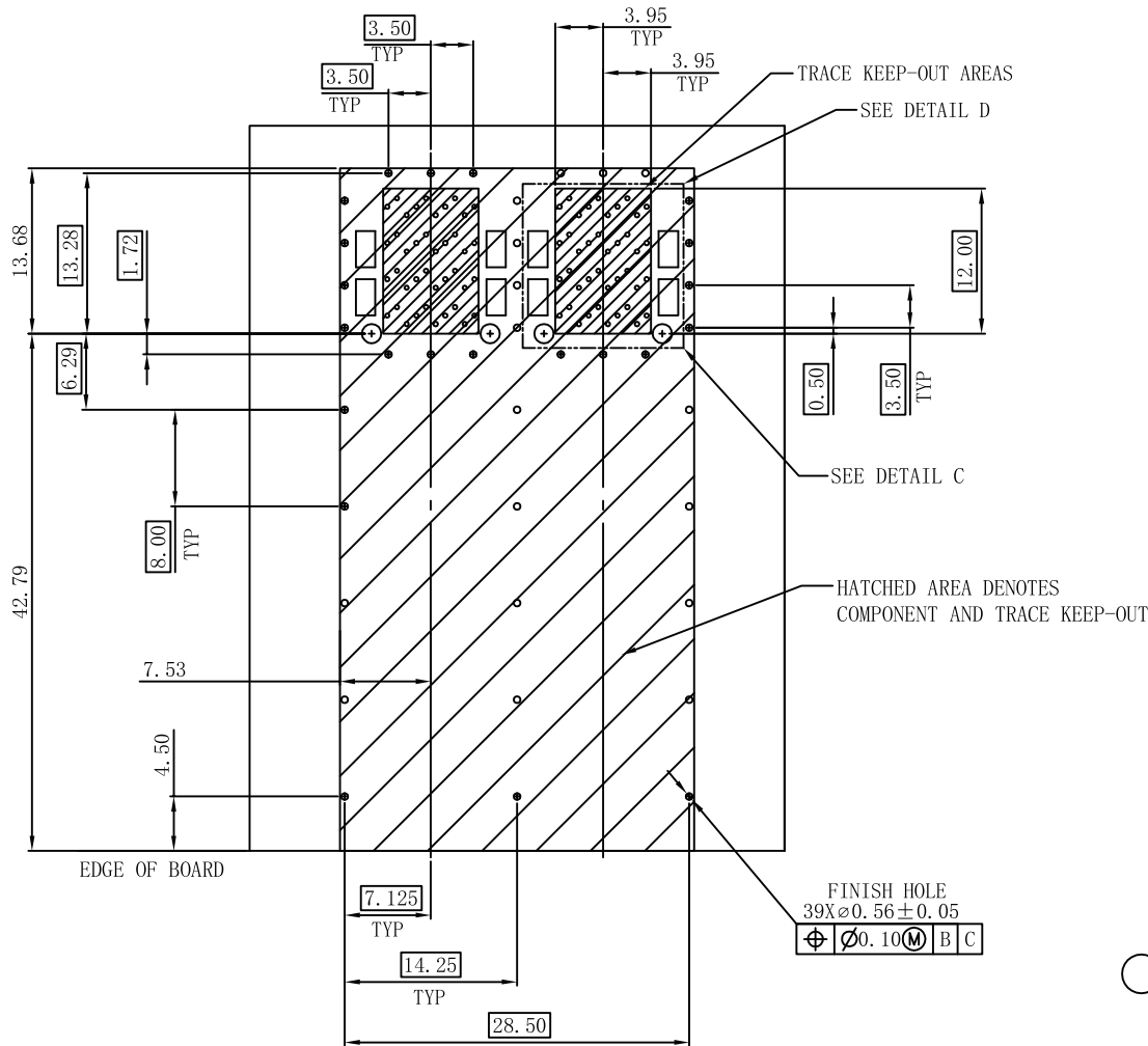
RECOMMENDED PCB LAYOUT-COMPONENT SIDE RECOMMENDED PCB THICKNESS-2.63mm
